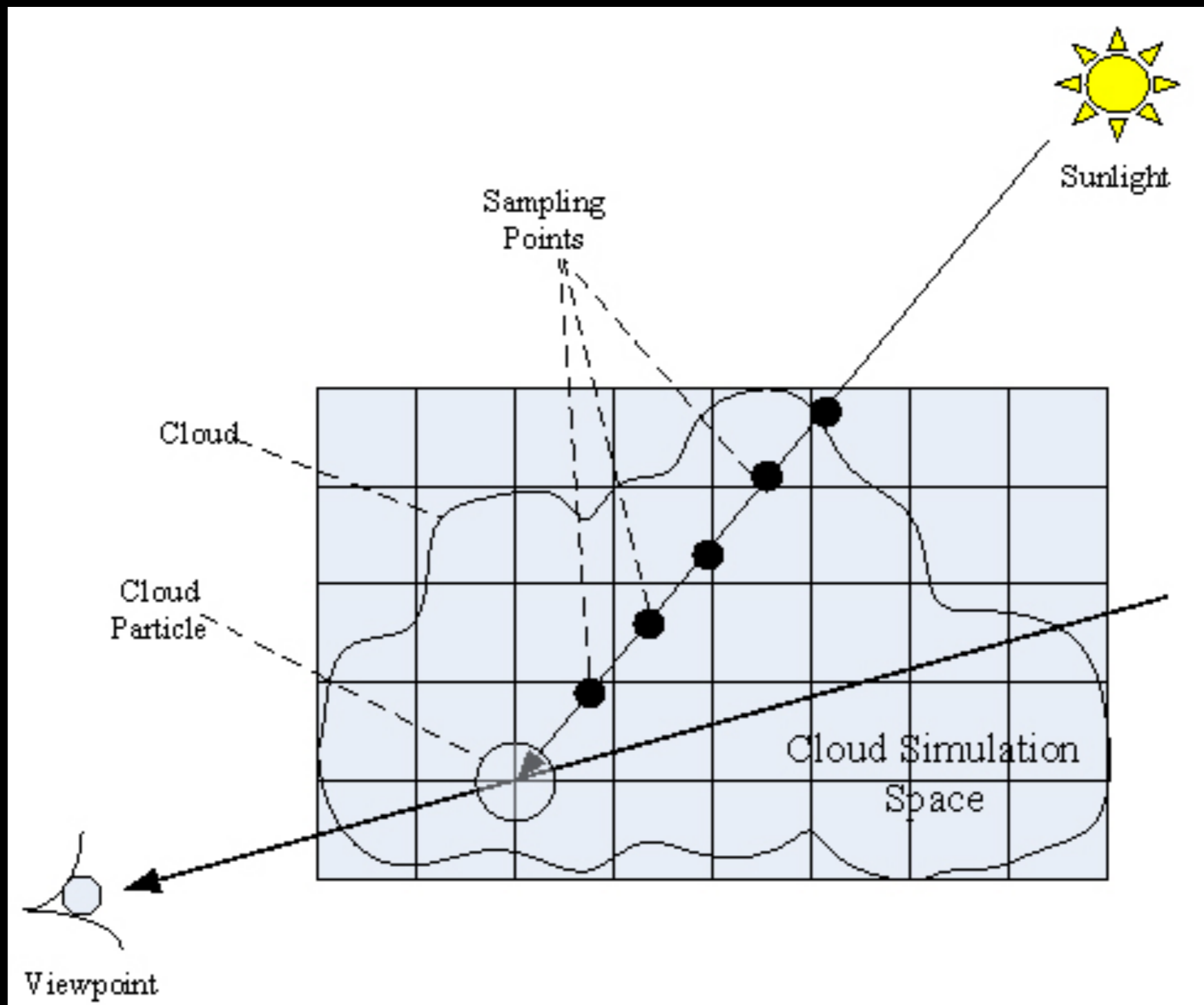
Cloud Particles
